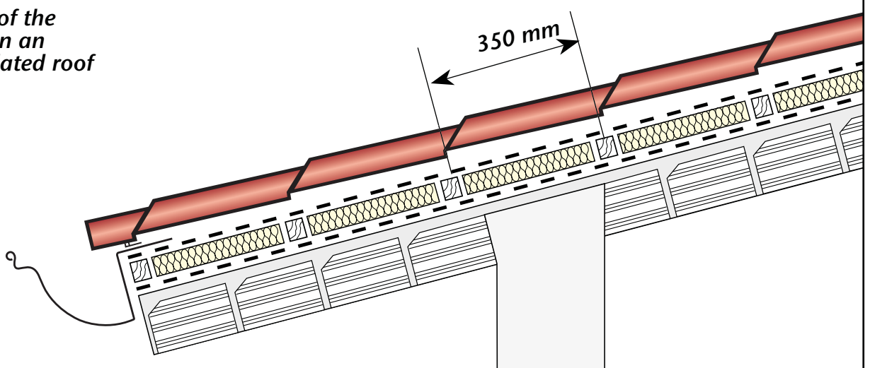
Ridge section on an unventilated roof
